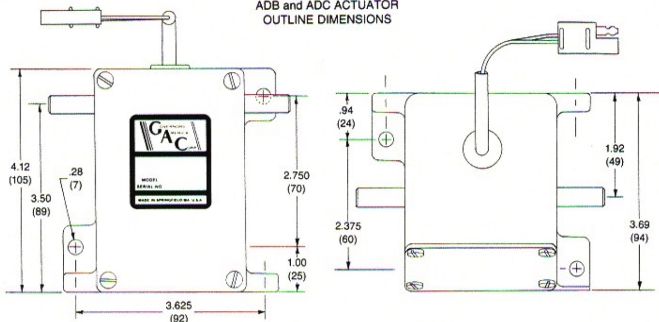
DIAGRAM 1b
